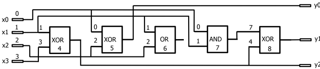
Fig. 1. A candidate circuit represented by CGP with parameters: n_i = 4 , n_o = 3 , n_c = 5 , n_r = 1 , l = 4 , \Gamma = \{0^{AND}, 1^{OR}, 2^{XOR}\} . Chromosome: 1, 3, 2; 0, 2, 2; 1, 2, 1; 0, 1, 0; 7, 4, 2; 5, 8, 4.
